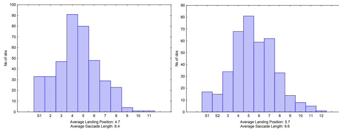
Figure 1. Landing distribution of the saccade originating from the target word (in letter positions). The letter S indicates a blank space. Left hand curve is the one blank space condition, right hand curve is the two blank spaces condition.
