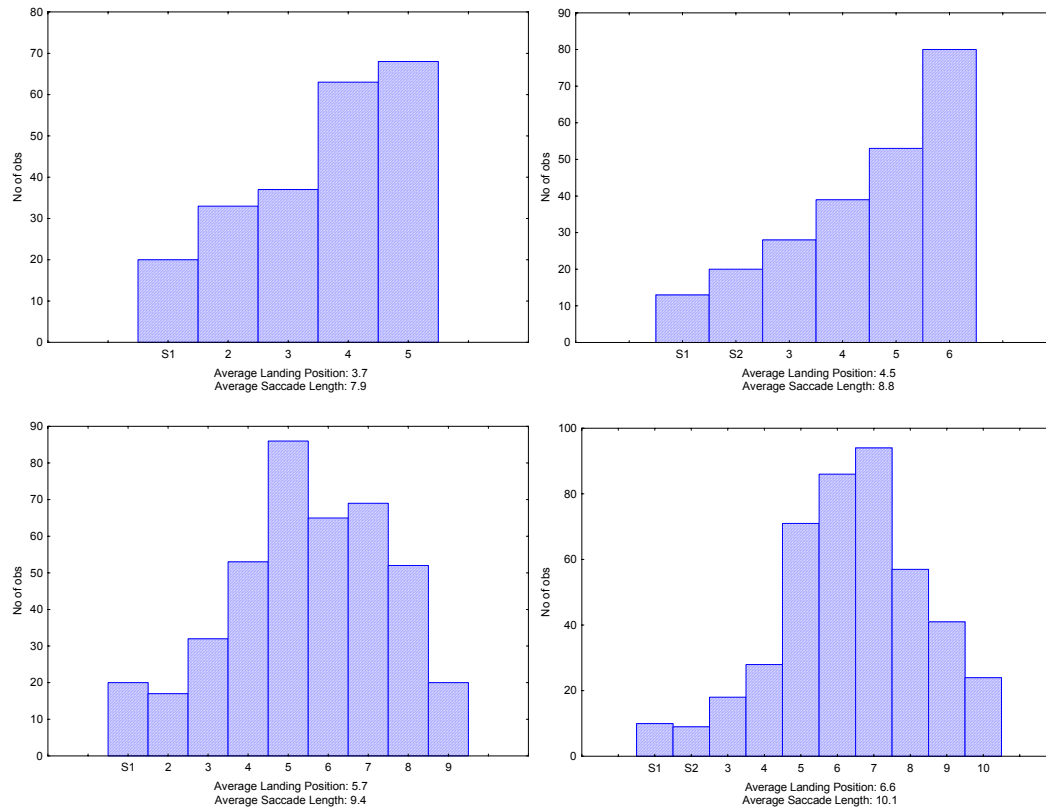
Figure 2. Landing distribution of the saccade originating from the target word (in letter positions) on the following word. The letter S indicates a blank space. The top curves are for the conditions with a 4 letter-word following the target word, the bottom curves are for the conditions with an 8 letter-word following the target word. Left hand curves are the one blank space conditions, right hand curve are the two blank spaces conditions.
